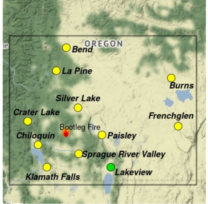
Daily AQI Forecast* for Aug 01, 2021
